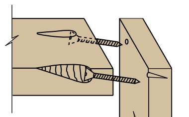
Pocket Screw
