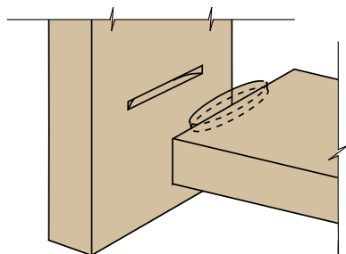
Biscuit Spline
